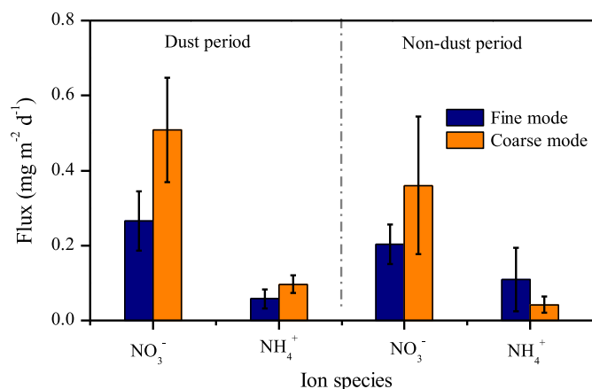
Fig. 7. The dry deposition flux of NO 3 - and NH 4 + in the fine (<2.1 μm) and coarse (>2.1 μm) modes during the dust storm events of 2017 in Xi'an, inland China.
