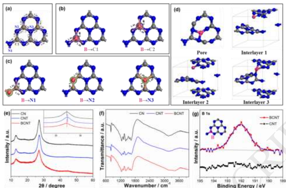
Fig. 1. (a) Pristine g\text{-C}_3\text{N}_4 mode. Boron atom substitution doping at (b) two inequivalent carbon sites or (c) three inequivalent nitrogen sites. (d) Interstitial doping at pore or interlayers. All samples underwent a subsequent geometry optimization. (e) XRD patterns (The small inset represents the (002) peaks of all samples after enlargement) and (f) FT-IR spectra of CN, CNT, and BCNT. (g) XPS high-resolution spectra of B 1s for BCNT and CNT.
