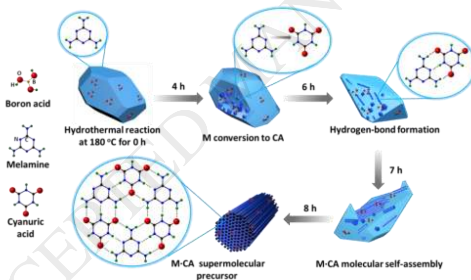
Scheme 1. Schematic diagram of the process of the BCNT precursor morphology evolution during the hydrothermal process with increasing reaction time.
