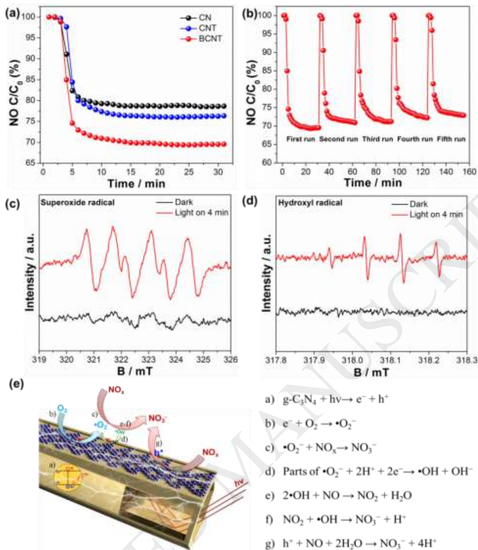
Fig. 5. (a) Visible light photocatalytic activities of CN, CNT, and BCNT for NO removal in air. (b) Cycling runs of BCNT. DMPO spin-trapping ESR spectra of BCNT (c) in methanol dispersion for DMPO-•O 2 - and (d) in aqueous dispersion for DMPO-•OH. (e) Schematic diagram of the photocatalytic NO x removal mechanisms with BCNT.
