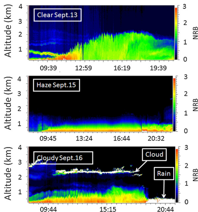
Fig. 2. Evolution of the PBL defined by the normalized relative backscatter (NRB, unit: count km 2 /( \mu s \mu j)) of MPL on clear sky (13 September, upper panel), haze (15 September, middle panel), and cloudy sky (16 September, lower panel) conditions.
